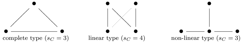
Fig. 3: connected components C such that r_C = 3
