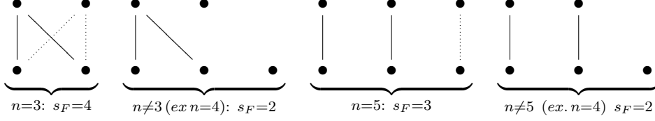
Fig. 2: linear types [2] , [2, 0, 0] , [1, 1, 1] and [1, 1, 0]
