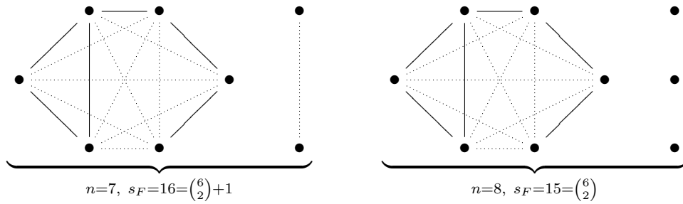
Fig. 1: graphs G_{\mathcal{B}} and G_{\mathcal{F}} for canonical subspaces of dimension 6 (the s_F - r edges of G_{\mathcal{F}} \setminus G_{\mathcal{B}} appear in dotted lines).
